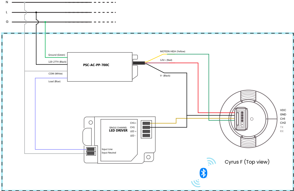
Dashed Line = 2x4 ft Fixture (Top view)
